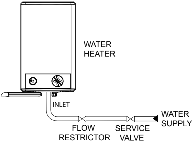
FIGURE 05 - PLUMBING DIAGRAM
